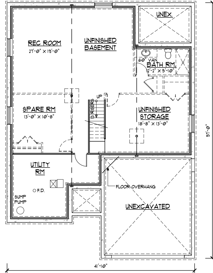
OPTIONAL BASEMENT FLOOR PLAN
