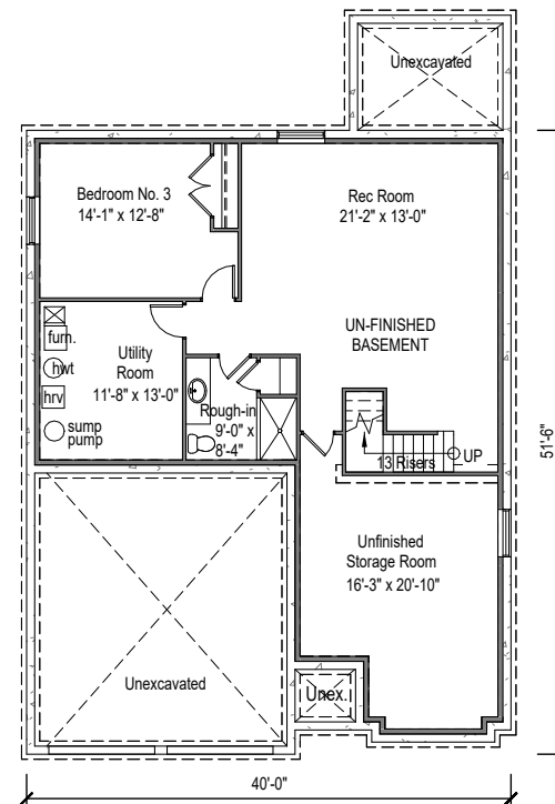
Optional Basement Floor Plan
