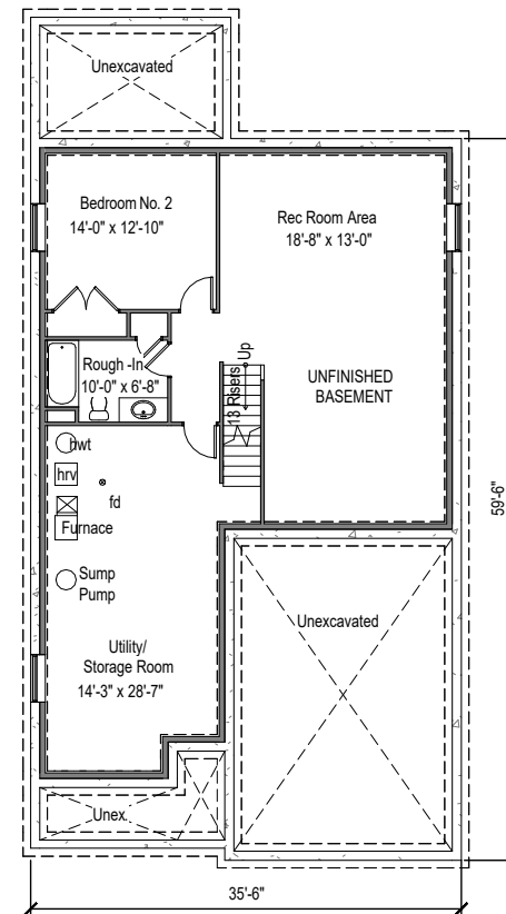
Optional Basement Floor Plan
