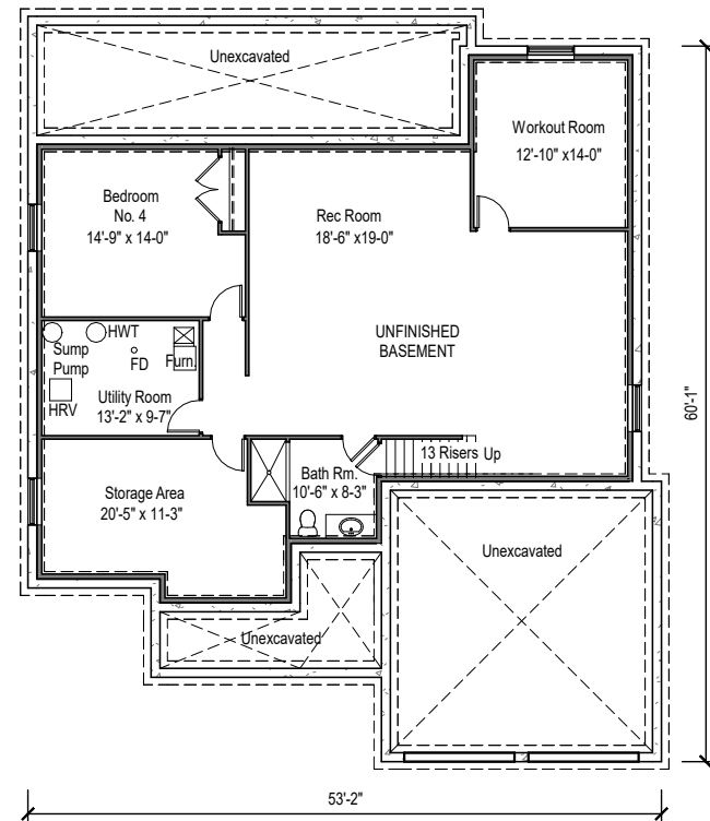
Optional Basement Floor Plan
