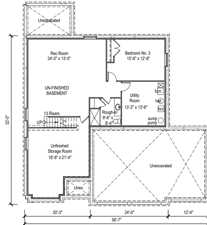
Optional Basement Floor Plan
