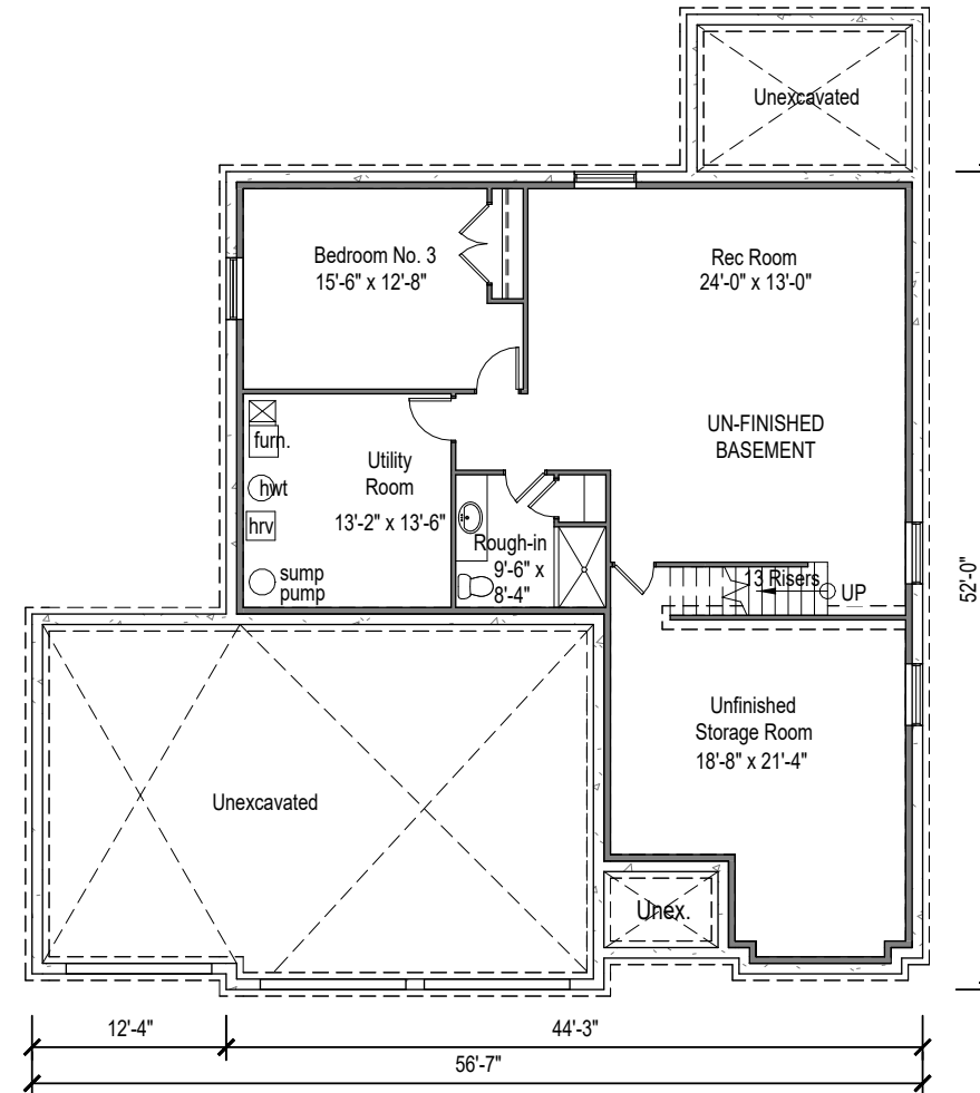
Optional Basement Floor Plan
