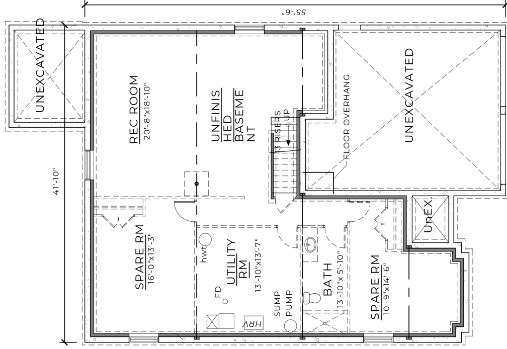
OPTIONAL BASEMENT FLOOR PLAN
