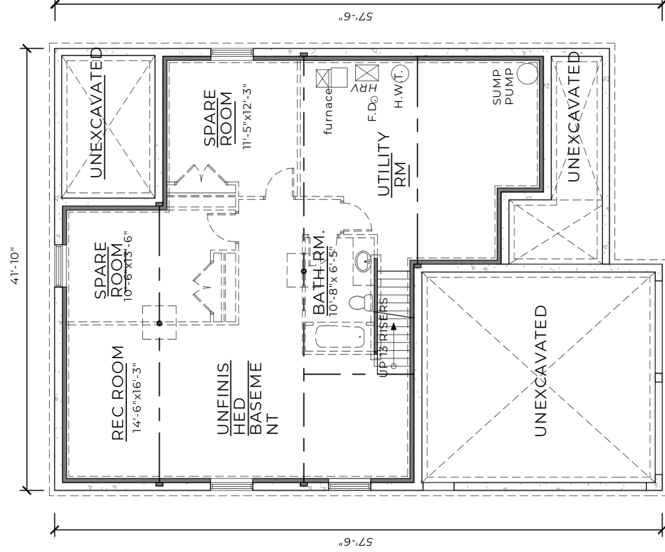
OPTIONAL BASEMENT FLOOR PLAN
