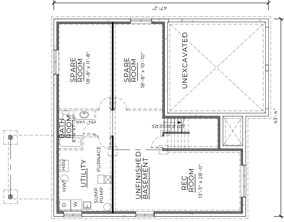
OPTIONAL BASEMENT FLOOR PLAN
