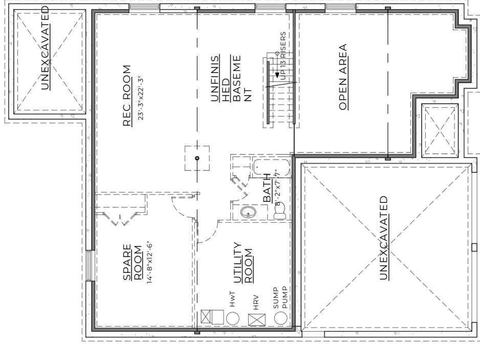
OPTIONAL BASEMENT FLOOR PLAN
