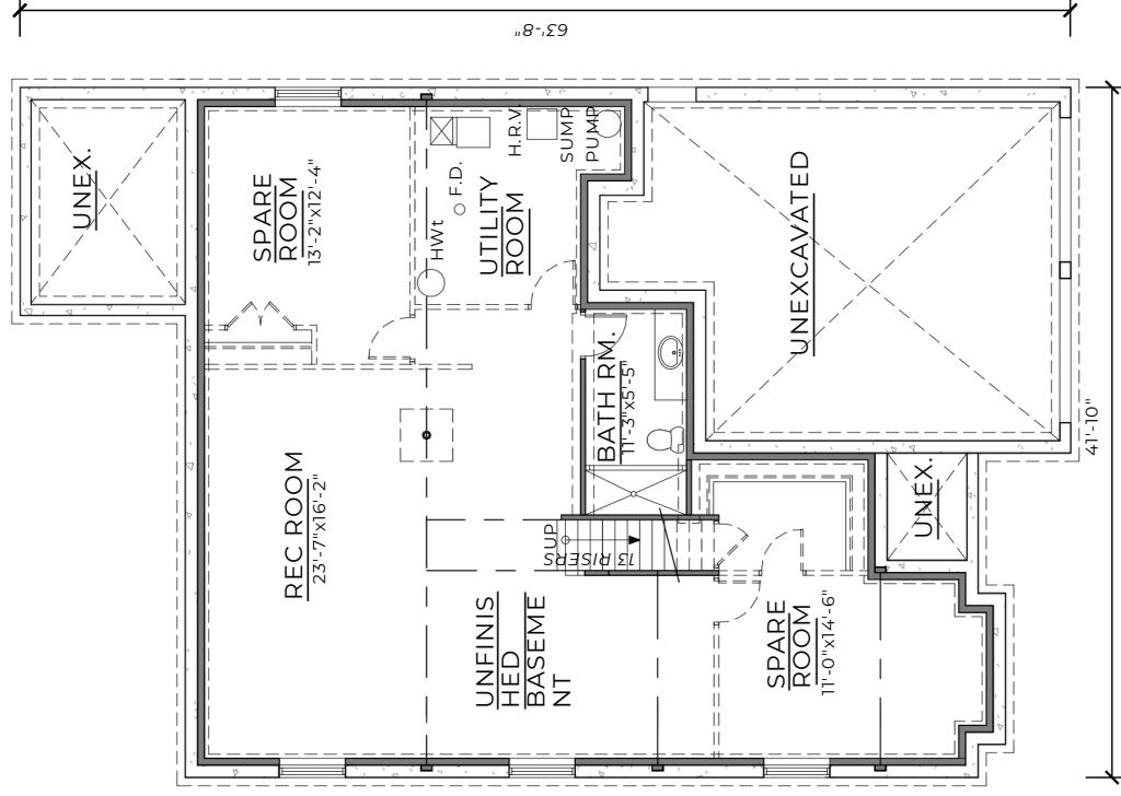
OPTIONAL BASEMENT FLOOR PLAN
